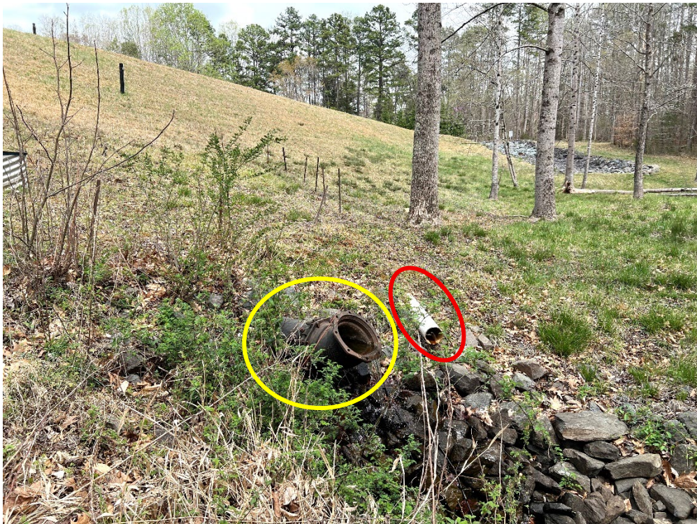
Photo 12 – Siphon Drain Outlet (To Remain Undisturbed – see yellow circle) and Seepage Collection PVC Pipe (To Be Removed – see red circle)
