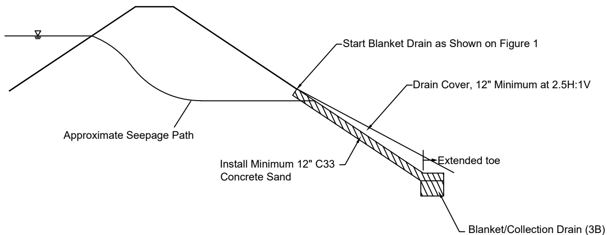
BLANKET DRAIN CROSS SECTION NTS
